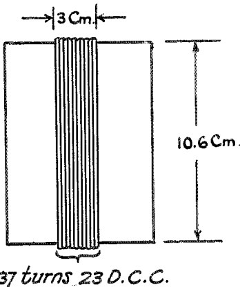
FIG. 23 Coils used in Figs. 15, 16 and 20.
