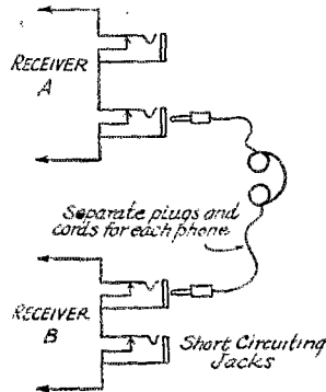
SIMPLE PLUG-JACK TRANSFER DUPLIX - TWO PHONES
